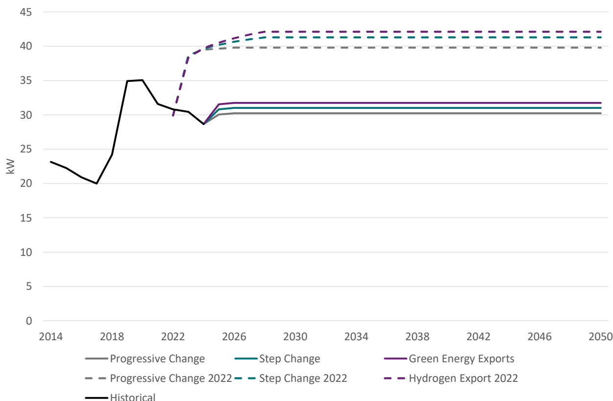
Figure 4-6 Historical and assumed future size of new commercial solar systems
