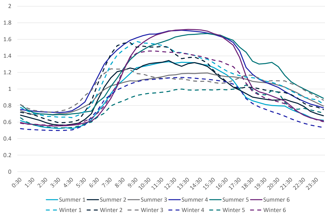
Apx Figure A.2 Index of average half hourly summer and winter loads for six commercial customers
