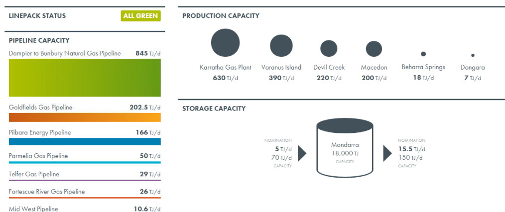
Figure 2.4: Linepack and Capacity Data
